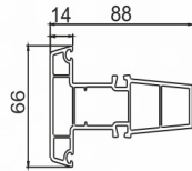
88 Transom Frame Mullion TC 88-3 (1.112 kg/m) 4 pieces/bag
