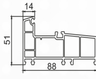
88 Transom Frame TC88-2 (1.082 kg/m) 4 pieces/bag
