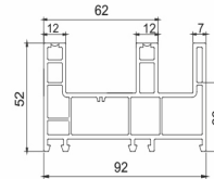
92 Sliding Frame TC92-1 (1.345 kg/m) 4 pieces/bag
