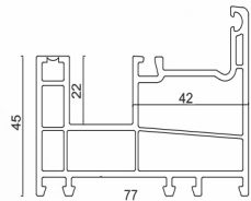
77 Mono Rail Frame TC80-17 (1.24 kg/m) 4 pieces/bag
