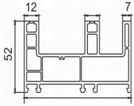
88 Sliding Frame TC88-1 (1.334 kg/m) 4 pieces/bag
