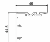
Interlock II 60 Sliding Door Sash TC 60-18 (0.25 kg/m) 20 pieces/bag
