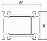
60 Universal Frame PC60-20 (0.81 kg/m) 8 pieces/bag
