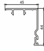
Interlock for 60 mm Door sash B TC 60-11B (0.255 kg/m) 20 pieces/bag
