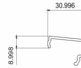
9 Villa Insect Bead PC60-24 (0.165 kg/m) 30 pieces/bag
