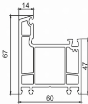
60 Casement Frame A PC60-1A (1.277 kg/m) 6 pieces/bag
