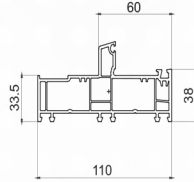
110 Villa Frame PC60-22 (1.51 kg/m) 4 pieces/bag
