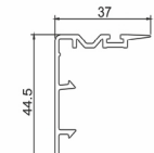
Interlock II 60 Sliding Big Window Sash TC 60-19 (0.24 kg/m) 20 pieces/bag
