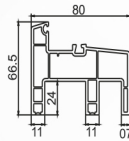
80 Integral Frame TC 80-5 (1.326 kg/m) 4 pieces/bag
