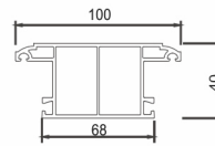
80 Door Mullion (Big) PM80-3 (0.969 kg/m) 4 pieces/bag
