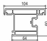
60 Outward Door Sash PM60-2 (1.527 kg/m) 4 pieces/bag
