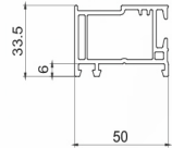
50 Add on track Villa window PC60-25 (0.65 kg/m) 8 pieces/bag
