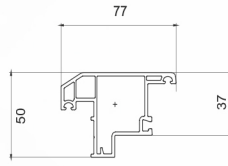
50 Villa Insect Sash PC60-23 (0.87 kg/m) 8 pieces/bag
