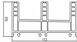
112 Three Sliding Track Frame II TC60-112 II (1.83 kg/m) 4 pieces/bag
