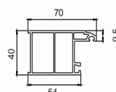
80 Small Door Sash PM80-10 (0.734 kg/m) 6 pieces/bag
